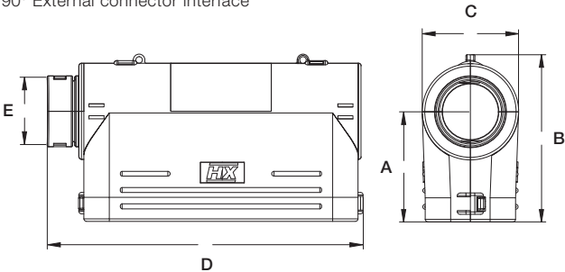
Dimensions 90° External connector interface
