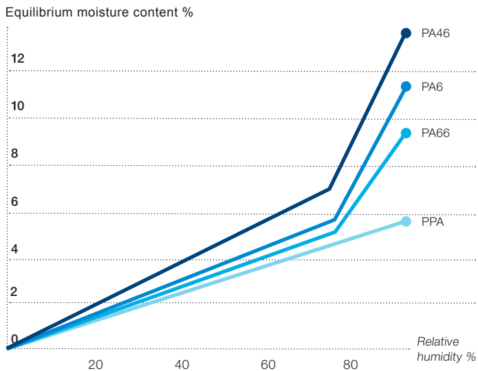
Figure 1. Moisture content of polyamides
