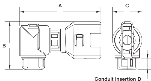
Dimensions GT153 elbow connector interface
