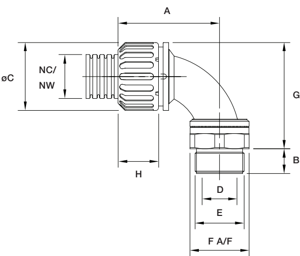
Dimensions 90° Elbow swivel fitting
