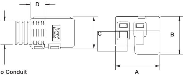
Dimensions External straight connector interface
